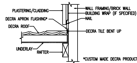
METHOD (iv) DECRA FLASHING INSTALLATION AT VERTICAL WALL JOINT
