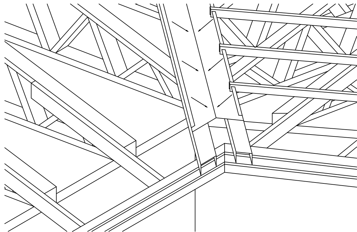
TWO 'C' SECTION STEEL
