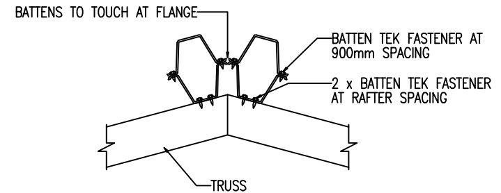
RIDGE BATTEN INSTALLATION
