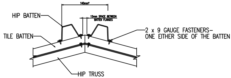
BARREL - HIP BATTEN INSTALLATION
