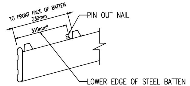
EAVE AND FIRST BATTEN LOCATION/SPACING
